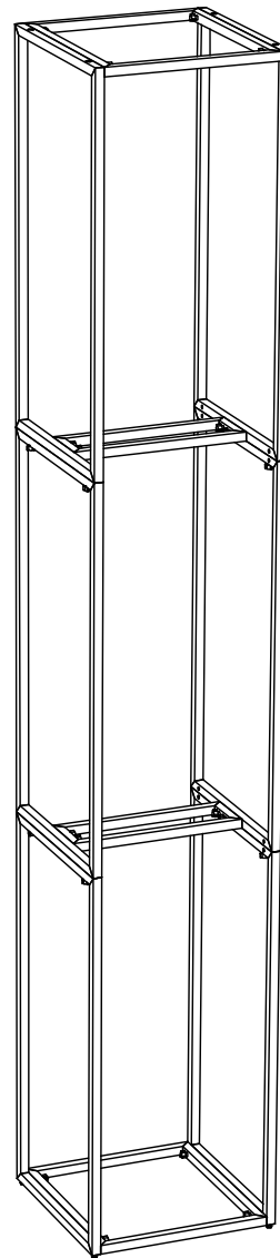
Frame dims: 23"W x 23"D x 138"H
