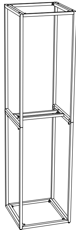
Frame dims: 23"W x 23"D x 92"H
