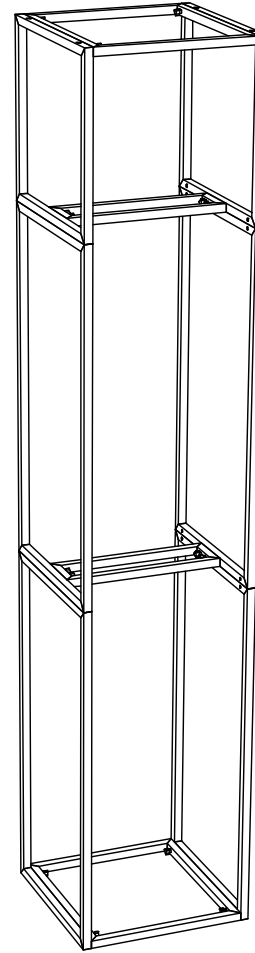
Frame dims: 23"W x 23"D x 115"H
