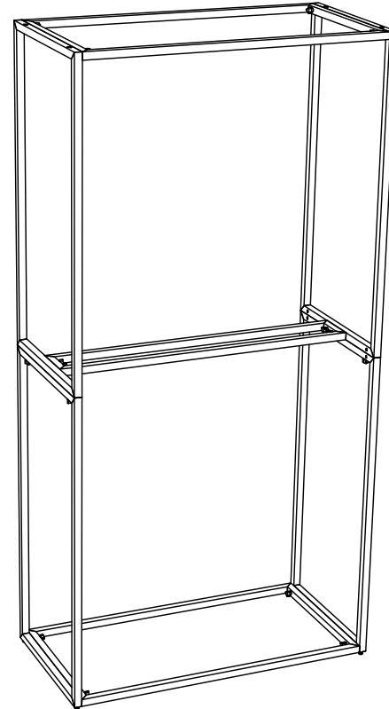
Frame dims: 46"W x 23"D x 92"H
