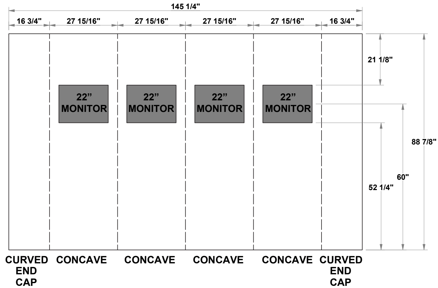
FLATTENED ELEVATED VIEW
