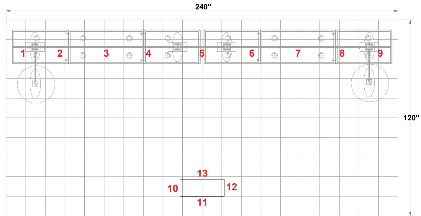
TOP VIEW
