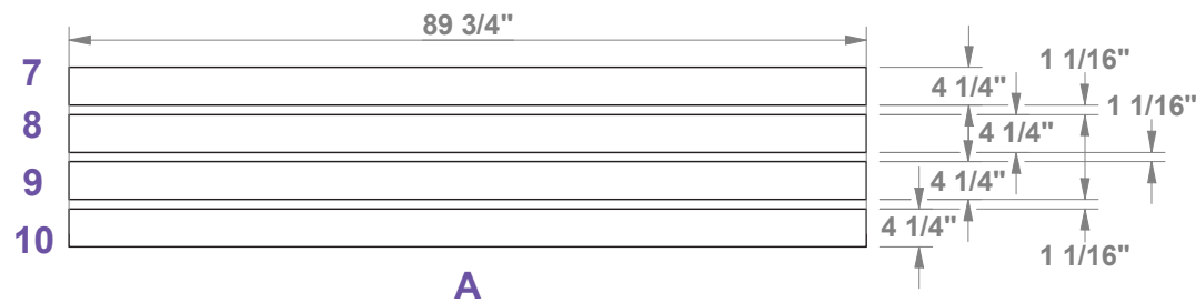
FLOOR PANELS - FLATTENED VIEW
